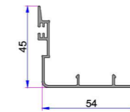
Alm. Kanat Arka Kapama 16051.601.5.1.1.9016
