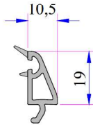
Triple Glazing Bead 30 mm Code: P.A.332.4100.600.0.HC
