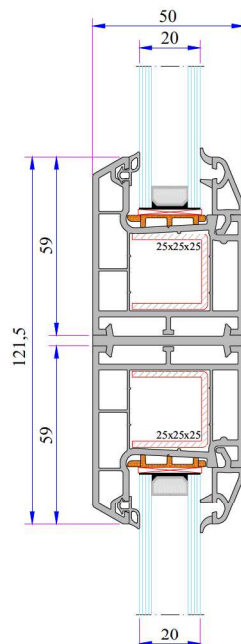
330 Frame - Narrow Coupling Profile
