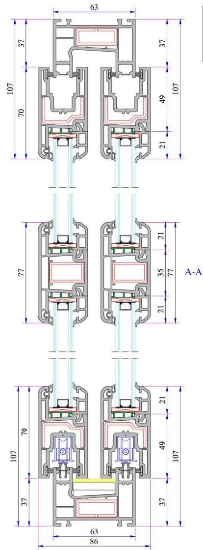
Mullion For Sash Installation
