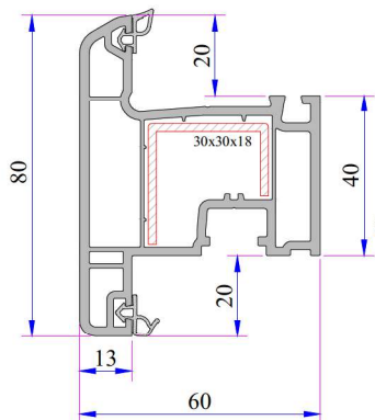
22 Axis Outward Opening Sash Profile
