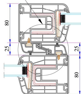
Hebeschiebe Sash Lap Strip Profile Installation
