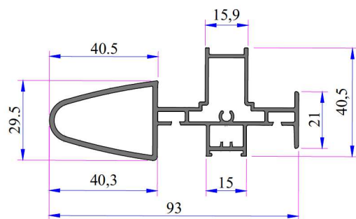
With Alum. Grillage Double Sash Middle Adaptor (In Process) Code: P.A.332.4000.600.0.HC
