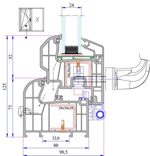
Frame-Sash Installation
