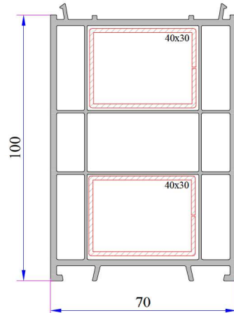
100mm Frame Lifting Profile
