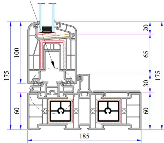
Hebeschiebe Sash and Rail Adaptor Installation
