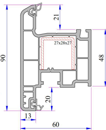
9 Axis Outward Opening Sash Profile Code: P.A.430.2001.600.0.BC.03
