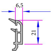
Triple Glazing Bead 42 mm
