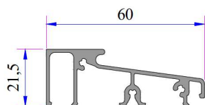
Seuil Aluminium Code: AD16-001
