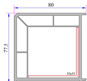
90° Corner Profile
