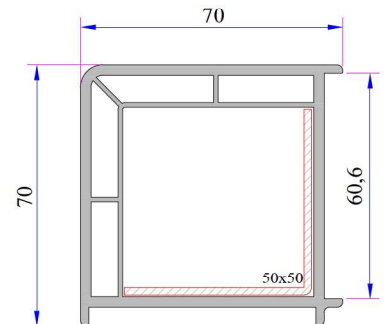
90° Corner Profile Code: P.A.060.5100.600.0.00.19
