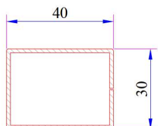
100mm Frame Lifting Profile Reinforcement Code: 34022-12120
