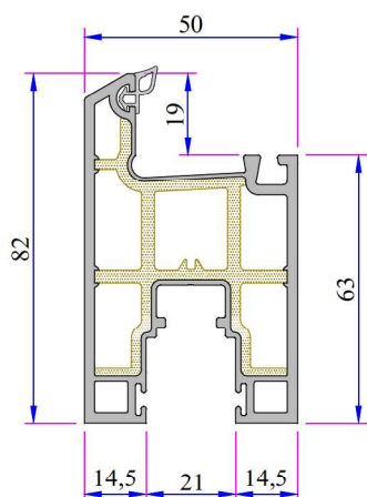
Sliding System Sash Profile Code: ???
