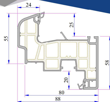
Offset Type Sash Profile Code: ???
