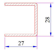
Outward Opening Sash Profile Reinforcement Code: 34022-12020
