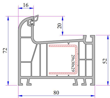
Frame Profile
