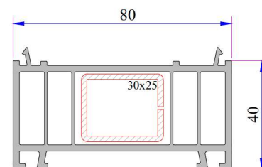
Frame Lifting Profile Code: P.A.080.5300.600.0.00.19
