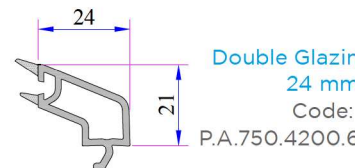
Outward Opening Door Sash Profile
