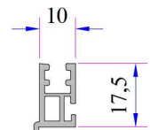
PVC Bumber Bead
