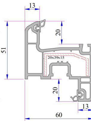
Narrow Sash Profile
