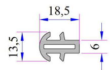
Short Coupling Profile Code: P.A.099.5003.600
