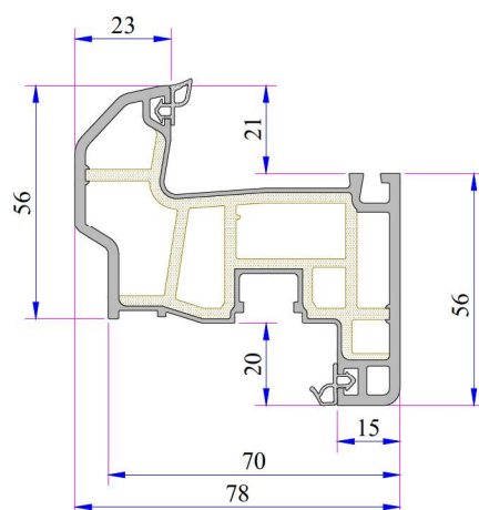
750 Penwood Offset Type Sash Profile Code: P.A.750.2200.600.2.BC.03
