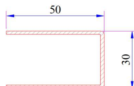
Door Sash- Outward Opening Door Sash Profile Reinforcement
