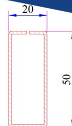
Large Coupling Profile Reinforcement Code: 34022-12105
