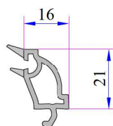
Decorative Triple Glazing Bead 32 mm
