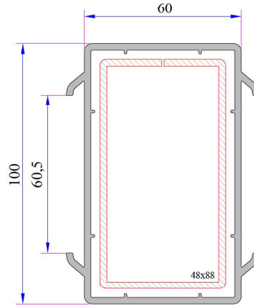
60x100 Box Profile
