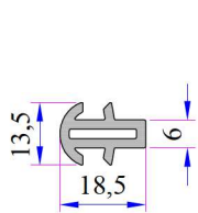
Coupling Profile
