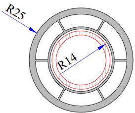
Angle Pipe Profile Code: P.A.050.5106.600
