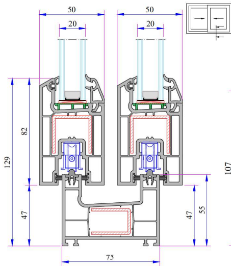
W 232 SLIDING SYSTEM WITH SINGLE RAIL SERIES
