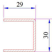
Sash - Offset Type Sash Profile Reinforcement Code: 34022-12002
