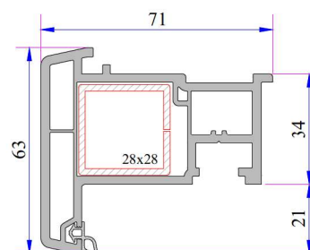
Lap Joint Profile Code: P.A.750.3100.600.0.BC.19
