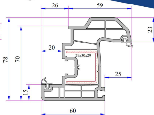
Offset Type Sash Profile
