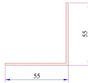
90° Corner Profile Reinforcement Code: 34022-12305
