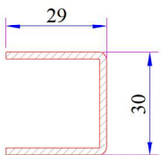
Frame - Sash - Offset Type Sash - Mullion Profile Reinforcement Code: 34022-12002
