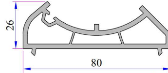
Angle Pipe Adaptor Profile
