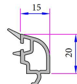
Triple Glazing Bead 42 mm
