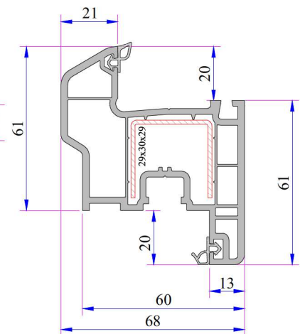
Offset Type Sash Profile
