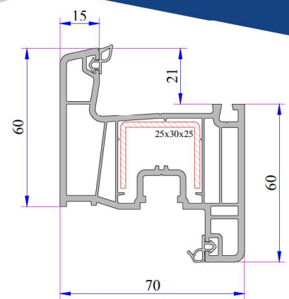
Sash Profile
