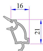
Double Glazing Bead 24 mm
