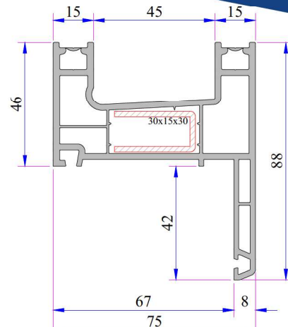
Frame Profile With Flat Sill Code: P.A.232.1110.600.0.00.03
