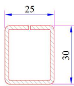
Mullion Profile Static Reinforcement Code: 34022-12119
