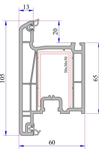
Outward Opening Door Sash Profile Code: P.A.642.2101.600.0.BC.03
