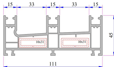
Frame Profile (Triple Rail) Code: P.A.222.1103.600.0.00.03
