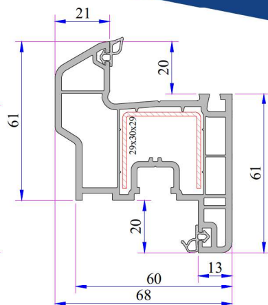
Offset Type Sash Profile Code: P.A.632.2200.600.0.BC.03
