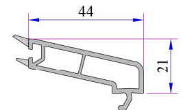
Single Glazing Bead 4-6 mm
