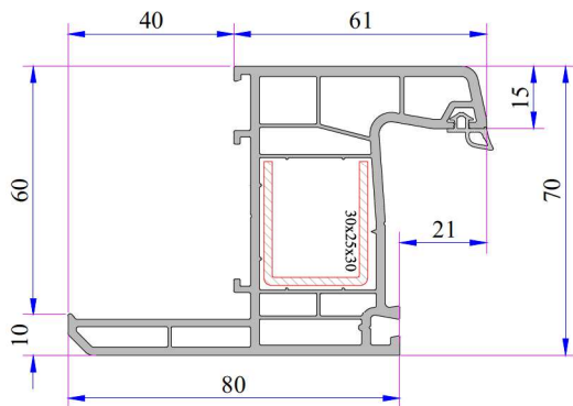
Frame Profile With Sill
