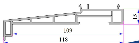
Sill Profile Code: P.A.058.5504.600.0.00.19
