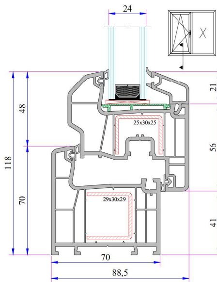
Frame - Offset Type Sash Installation
