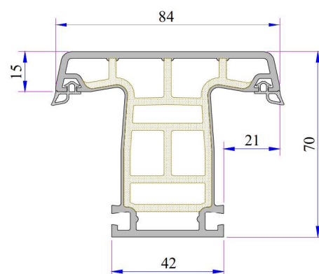
750 Penwood Mullion Profile Code: P.A.750.3000.600.2.BC.03
