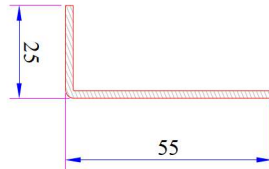
135° Corner Profile Reinforcement Code: 34022-12303
