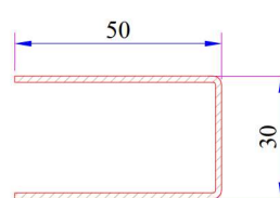
Door Sash - Outward Opening Door Sash Reinforcement
