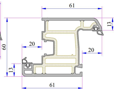
760 Penwood Sash Profile Code: P.A.632.2000.600.2.BC.03
