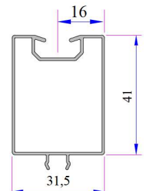
Shutter Side Rail Lifting Profile
