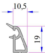
Triple Glazing Bead 30 mm
