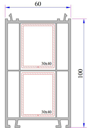
60x100 Frame Lifting Profile
