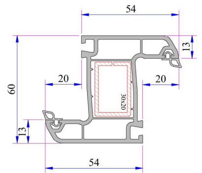
Outward Opening Mullion Profile
