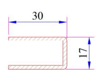
Frame Profile with Sill Reinforcement
