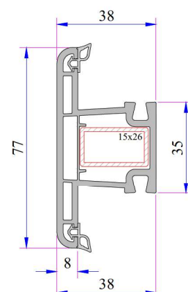
Mullion Profile for Sash Profile Code: P.A.222.3201.600.0.BC.03
