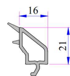
Double Glazing Bead 24 mm
