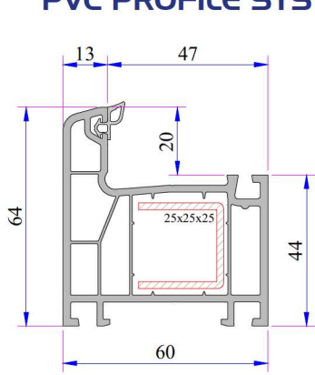
Frame Profile
