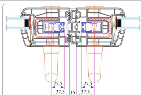
Sash and Rail Adaptor Installation
