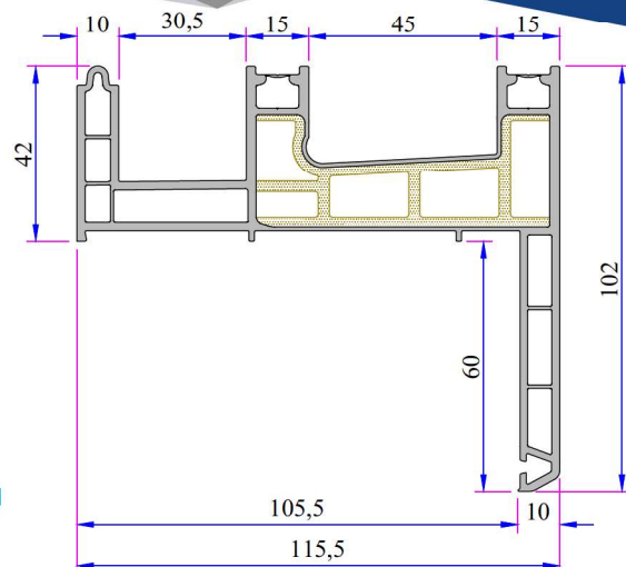
Penwood Frame With Fly-Screen&Sill Code: ???
