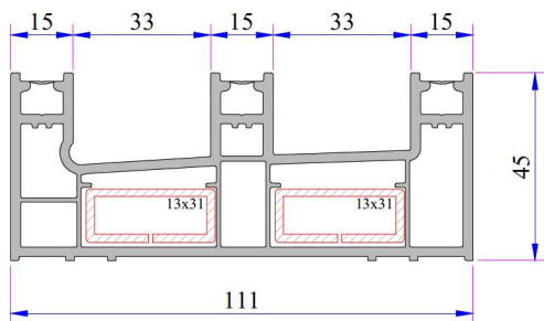
New Frame Profile (Triple Rail) Code: P.A.222.1112.600.0.00.03
