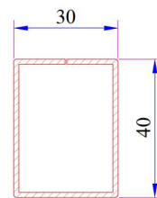
100mm Frame Lifting Profile Reinforcement Code: 34022-12120
