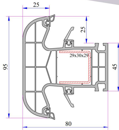
Mullion Profile
