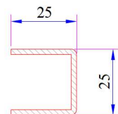
24 Axis. Sash Profile Reinforcement Code: 34022-12003
