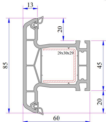
Mullion Profile
