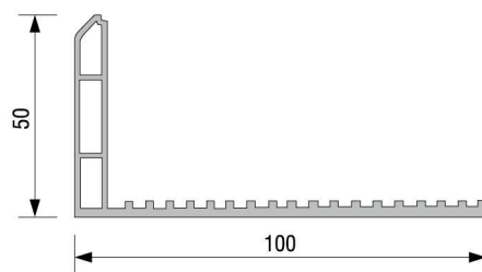
Panel Profile (50x100) Code: P.A.099.5501.600.0.00.19
