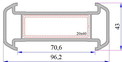
Large Coupling Profile
