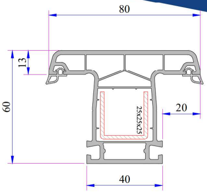
Mullion Profile
