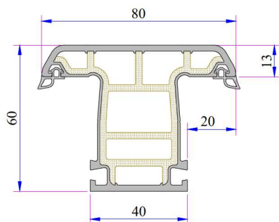
632 Penwood Mullion Profile Code: P.A.632.3000.600.2.BC.03
