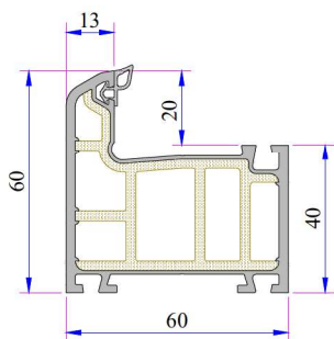
632 Penwood Frame Profile Code: P.A.632.1000.600.2.BC.03
