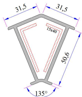
Corner Profile (135°)
