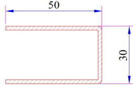
Door Sash - Outward Opening Door Sash Profile Reinforcement Code: 34022-12013
