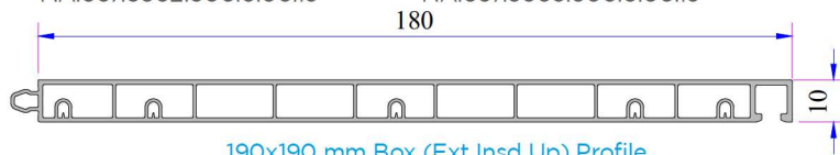
190x190 mm Box (Ext Insd Up) Profile
