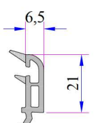
Triple Glazing Bead 42 mm
