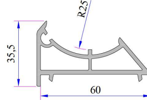
Corner Lag Profile
