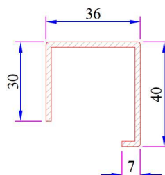
Sliding System Sash Profile (Static) Reinforcement Code: 34022-12107
