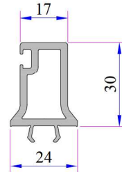
Hebeschiebe Frame Middle Adaptor Code: P.A.900.6503.600
