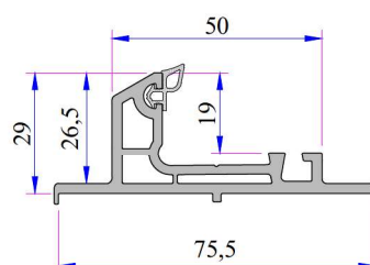
Double Rail Adaptör Profile Code: P.A.232.5800.600.0.BC.19
