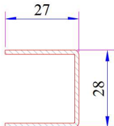
Outward Opening Sash Profile (9 Axis) Reinforcement Code: 34022-12020
