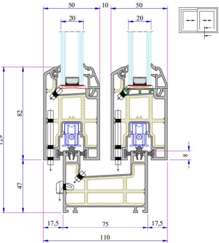
Sliding Frame Sash Double Rail Installation
