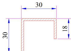
22 Axis Outward Opening Sash Profile Reinforcement
