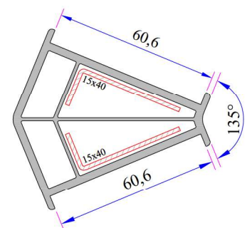
135° Corner Profile
