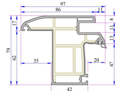
632 Penwood Shutter Rail Frame Profile Code: P.A.632.1206.600.2.BC.03
