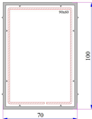
70x100 mm Box Profile
