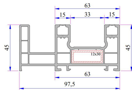
Frame With Fly-Screen Code: ???
