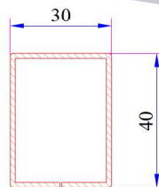
100 mm Frame Lifting Profile Reinforcement Code: 34022-12120
