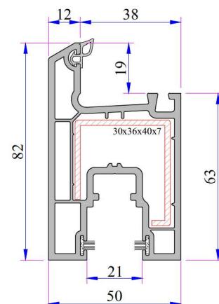
Sliding System Sash Profile (Static) Code: P.A.232.2308.600.0.BC.03
