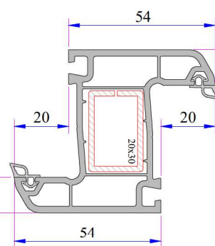
Outward Opening Mullion Profile
