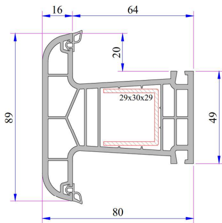
800 Series Mullion Profile Code: P.A.860.3000.600.0.00.BC.03
