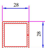
Lap Joint Profile Reinforcement Code: 34022 - 12113
