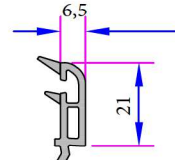
Double Glazing Bead 17 mm Code: P.A.532.4500.600.0.HC
