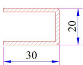
Frame Profile with Sill 60mm Reinforcement
