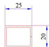
35mm Frame Lifting Profile Reinforcement Code: 34022-12104
