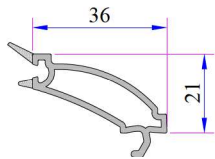
Single Glazing Bead 4-6 mm
