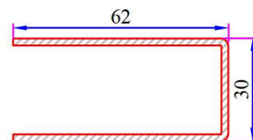
Super Door Sash Profile Reinforcement Code: 34022 - 12029
