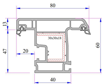
22 Axis. Outward Opening Sash Profile Code: P.A.632.2014.600.0.BC.03
