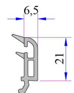
Triple Glazing Bead 42 mm
