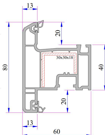
22 Axis Outward Opening Sash Profile Code: P.A.632.2014.600.0.BC.03
