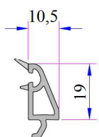
Triple Glazing Bead 30 mm
