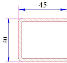
Hebeschiebe Sash Profile Reinforcement Code: 34022-25001
