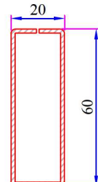
Large Coupling Profile Reinforcement Code: 34022 - 12106
