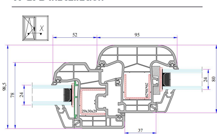
Mullion - Offset type sash Installation
