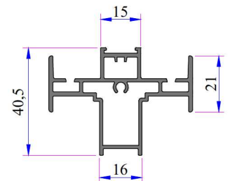
With Alum. Lug Double Sash Middle Adaptor (In Process) Code: ??
