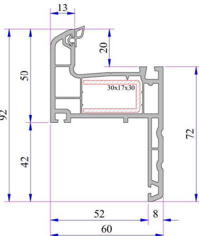
Frame Profile with Sill
