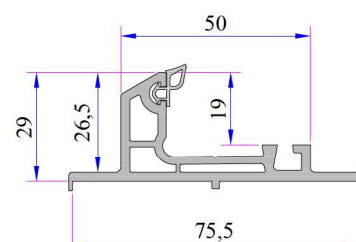
Double Rail Adaptor Profile Code: P.A.232.5800.600.0.BC.19
