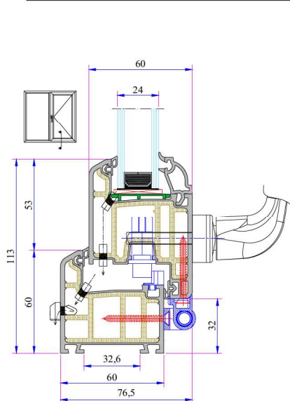
Frame-Sash Installation
