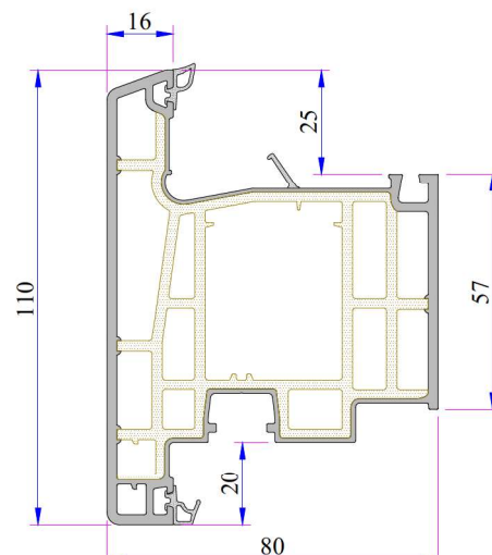
Outward Opening Door Sash Profile Code: ???
