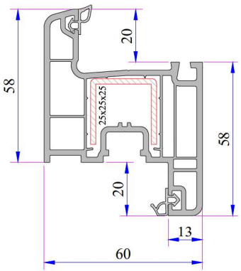
Sash Profile
