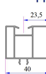
Shutter Side Rail Lifting Profile Code: 21108-01000
