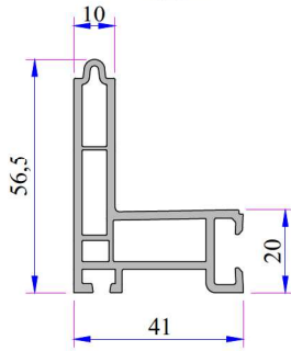
Screen Adaptör Profile Code: P.A.232.5802.600.0.00.19
