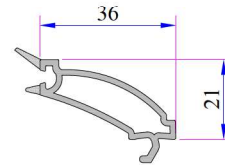
Single Glazing Bead 4-6mm
