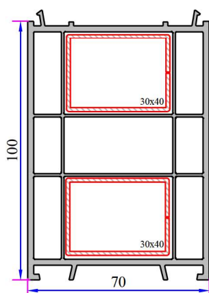
Frame Lifting Profile
