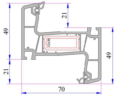
Outward Opening Mullion Profile
