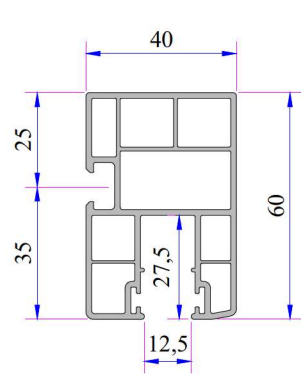
37 mm Blade Side Rail
