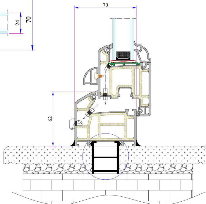
Offset Profile and Frame Montage Profile Installation
