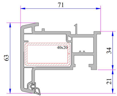
Static Lap Joint Profile (Spiked)
