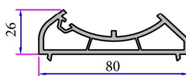
Corner Lag Profile
