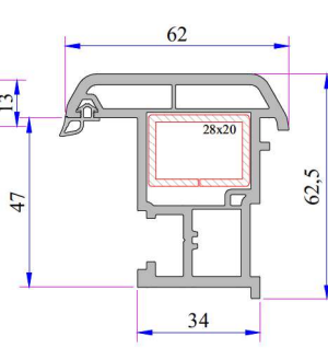
Lap Joint Profile Code: P.A.632.3100.600.0.BC.19
