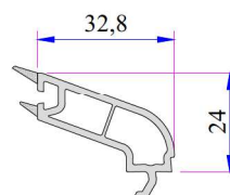
Glazing Bead 24mm Code: ???
