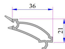
4 mm Glazing Bead Code: P.A.101.4002.600.0.HC
