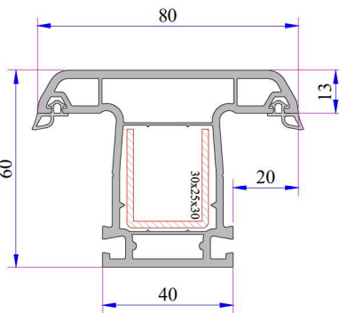
Mullion Profile
