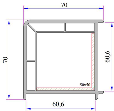
90° Corner Profile
