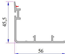
Sash Cover Profile Code: P.A.222.8700.600
