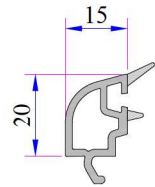
Triple Glazing Bead (42mm) Code: P.A.800.4600.600.0.HC
