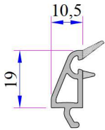
Double Glazing Bead (20mm) Code: P.A.332.4100.600.0.00.HC
