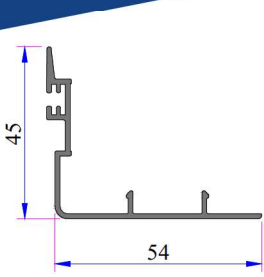
Alum. Sash Cover Profile Code: 16051.601.5.1.1.9016
