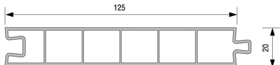
Panel Profile (125) Code: P.A.099.5404.600.0.00.19
