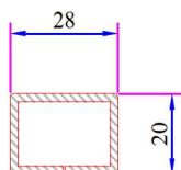
Lap Joint Profile Reinforcement Code: 34022 - 12118
