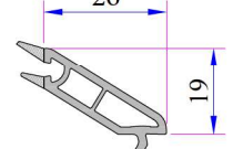
4mm Single Glazing Bead
