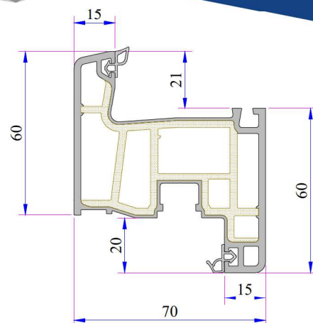
750 Penwood Sash Profile Code: P.A.750.2000.600.2.BC.03
