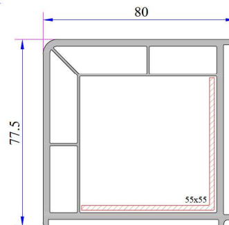
90° Corner Profile
