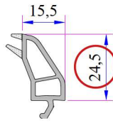
Triple Glazing Bead 32 mm
