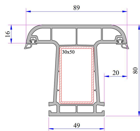
Static Mullion Profile
