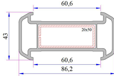
Large Coupling Profile
