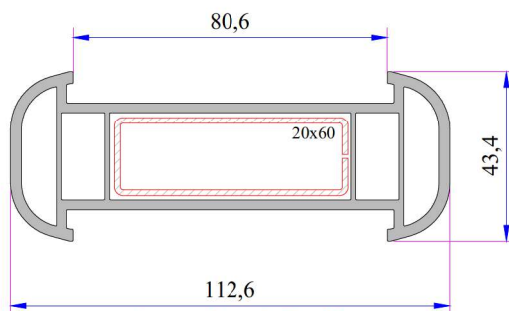
Large Couple Profile Code: P.A.080.5000.600.0.00.19
