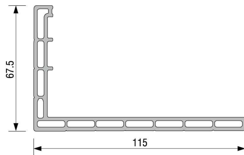
Frame Panel Profile Code: P.A.099.5505.600.0.00.19
