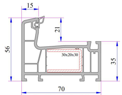
Eco Frame Profile
