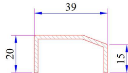
Narrow Sash Profile Reinforcement Code: 34022-12031
