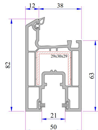
Sliding System Sash Profile Code: P.A.232.2300.600.0.BC.03
