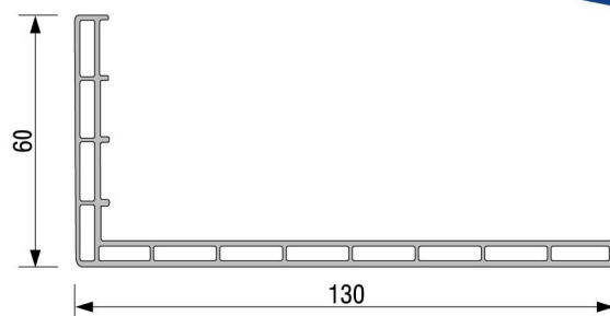
60x130 Border Profile Code: P.A.099.5503.600.0.00.19
