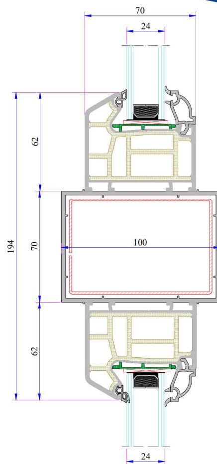
Box Profile Installation
