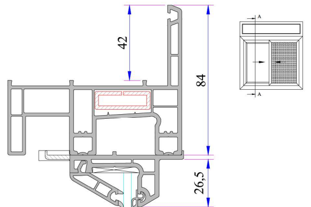
Double Rail Adaptor Profile Installation
