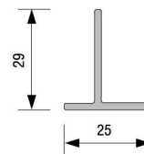
T Profile Code: P.A.099.5507.600
