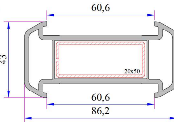
Large Coupling Profile Code: P.A.060.5000.600.0.00.19
