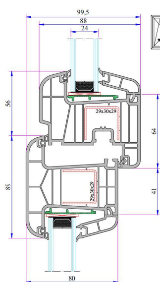
Sash - Mullion Profile Installation
