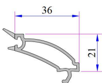
Single Glazing Bead 4-6 mm
