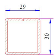
Mullion Profile Static Reinforcement Code: 34022-15129
