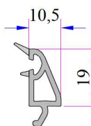
20mm Double Glazing Bead
