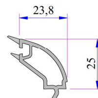
Glazing Bead 32-34mm Code: P.A.777.4204.600.0.HC
