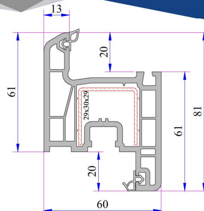
Sash Profile
