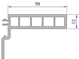
Frame Sill Profile (50mm) Code: P.A.099.5524.600
