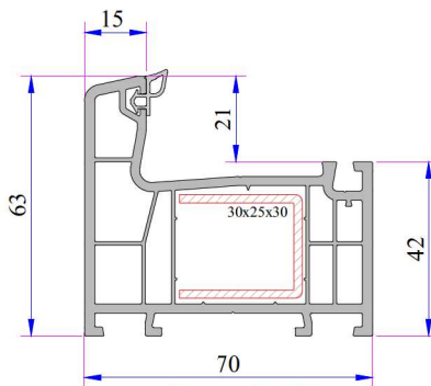
Frame Profile
