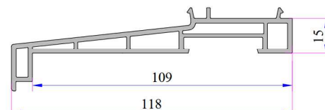
Sill Profile Code: P.A.058.5504.600.0.00.19
