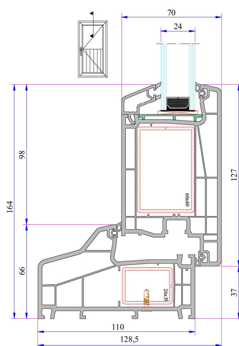
Frame - Outward Opening Super Door Sash Installation
