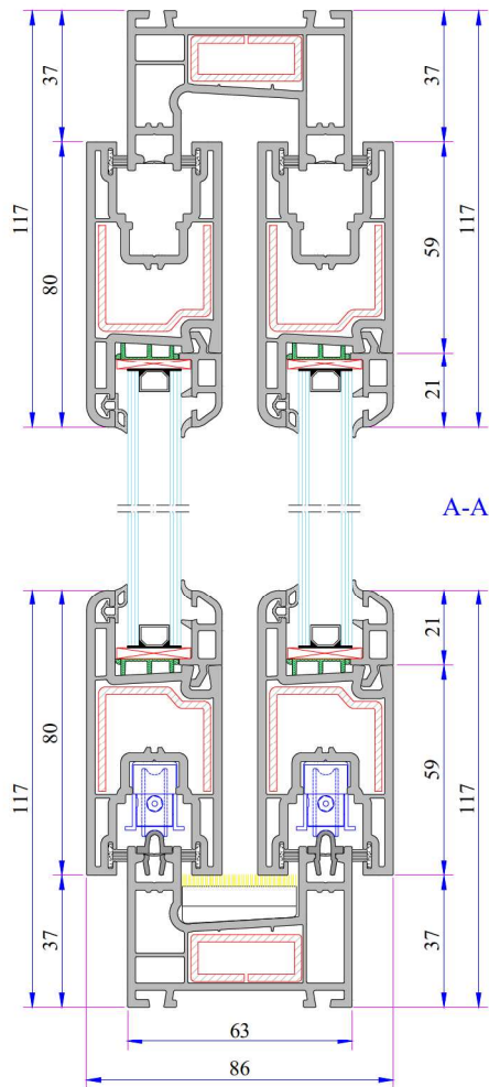
Double Railed Frame and Double Sash Installation
