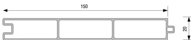
Panel Profile Code: P.A.099.5407.600.0.00.19
