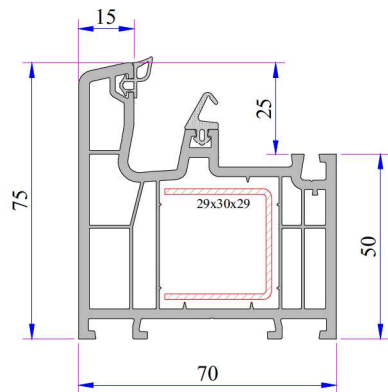
Frame Profile
