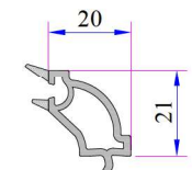
Dec. Double Glazing Bead 28 mm
