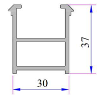
Frame Montage Profile Code: P.A.060.5301.600.0.00.19
