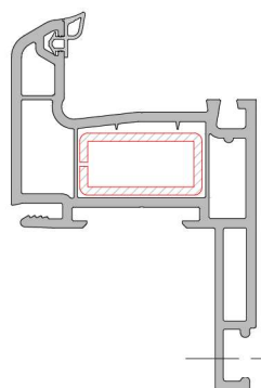
135° Corner Profile Installation
