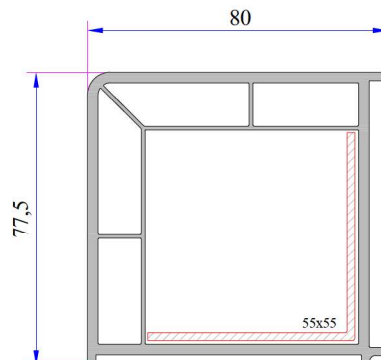
90° Corner Profile
