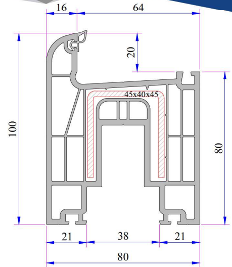
Hebeschiebe Sash Profile Code: P.A.930.2301.600.0.00.BC.03
