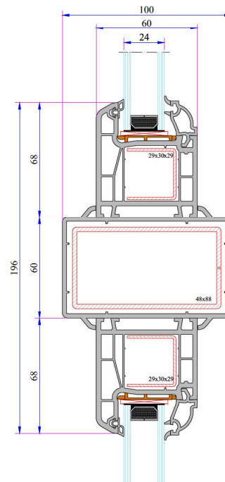
60x100 Spiked Box Profile Installation
