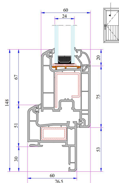
30mm Frame With Sill - Eco Door Sash Installation
