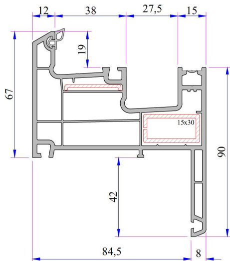
Frame Profile With Sill (Single Rail) Code: P.A.232.1114.600.0.00.03
