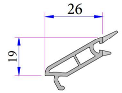
Single Glazing Bead (4mm) Code: P.A.332.4000.600.0.00.HC
