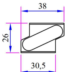
Single Sled Code: 34020-11010
