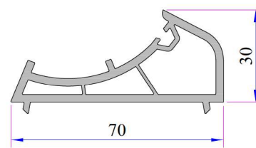
Corner Lag Profile
