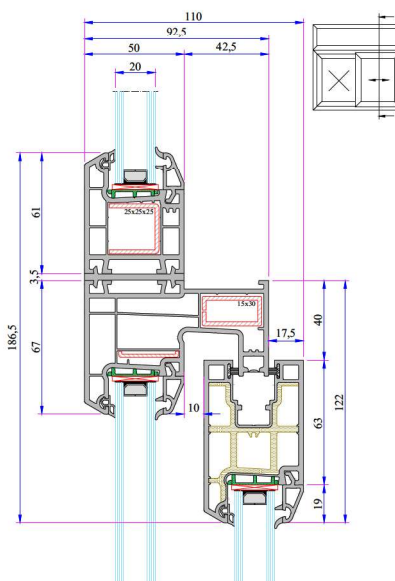
Top Fixed - Bottom Single Rail Sliding Installation
