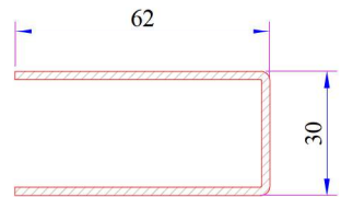
Super Door Sash Profile Reinforcement Code: 34022-12029
