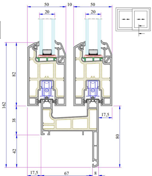
Double Sliding Frame with Sill - Sash Installation
