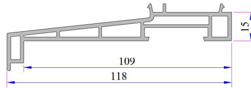
Sill Profile Code: P.A.058.5504.600.0.00.19
