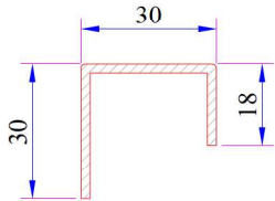
22 Axis. Outward Opening Sash Profile Reinforcement Code: 34022-12022
