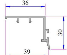
Sash Cover Profile
