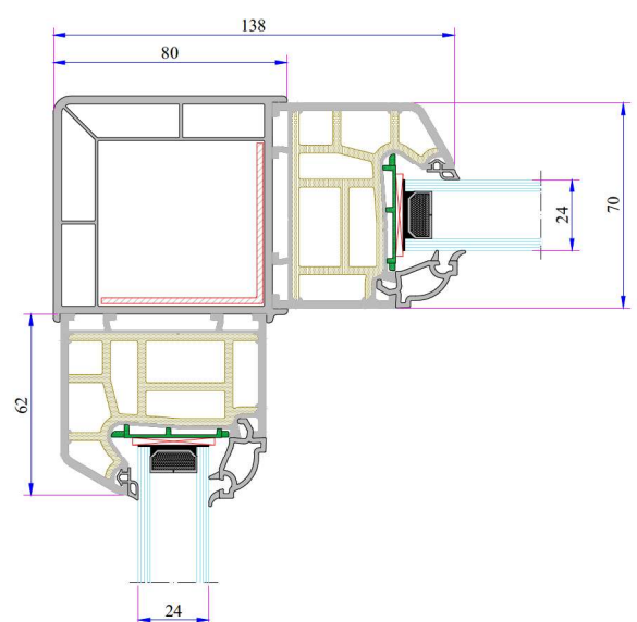
90° Corner Installation
