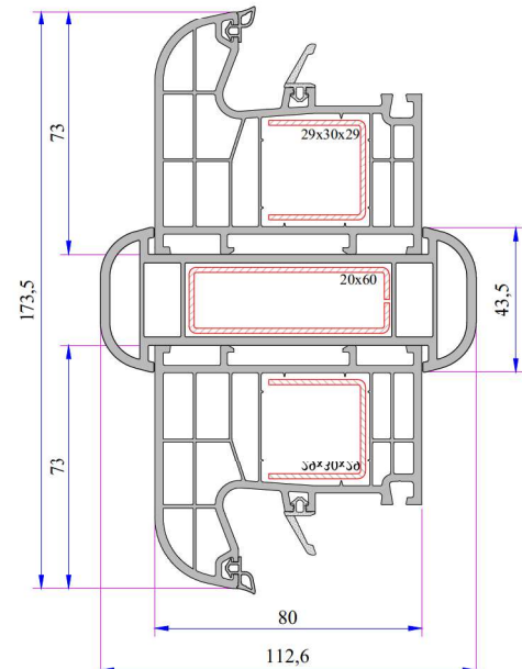
Large Coupling Profile Installation
