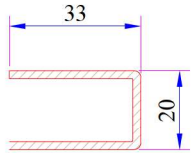
Sliding Frame Profile Reinforcement Code: 34022-12019
