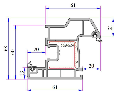
Offset Type Sash Profile Code: P.A.632.2200.600.0.BC.03
