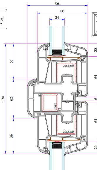
Sash - Lap Joint Installation
