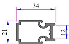
Alum. Double Rail Adaptor Profile Code: AD16-011(White)
