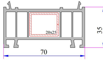
35mm Frame Lifting Profile Code: P.A.070.5300.600.0.00.19
