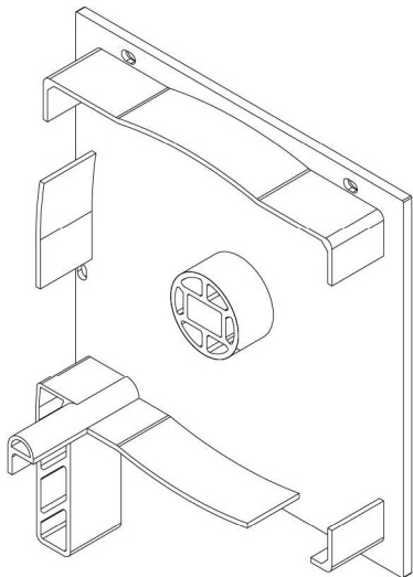
155x155 mm Motorized Shutter Side Cover (Right And Left Sides Are The Same) Code: 34019-11050
