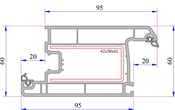
Super Door Sash Profile Code: P.A.632.2100.600.0.BC.03
