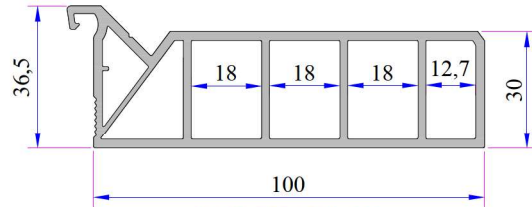
WF - FOUR \ 100 Code: P.A.900.6308.600.0.00.19
