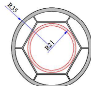
Pipe Profile
