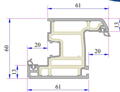
632 Penwood Sash Profile Code: P.A.632.2000.600.2.BC.03
