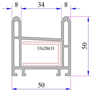
Sliding Frame Profile
