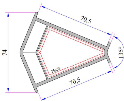
135° Corner Profile
