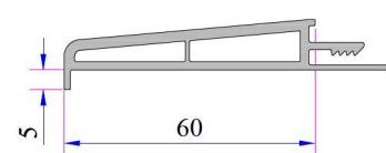
Sill Profile Under Frame (60mm)
