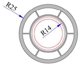
Pipe Profile
