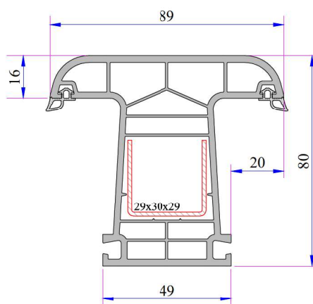
Mullion Profile
