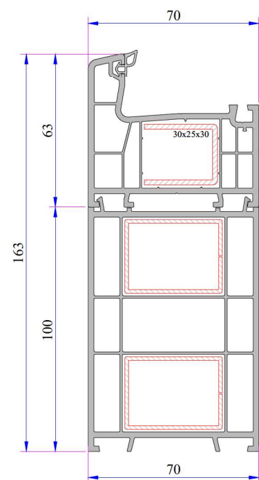
100mm Frame Lifting Profile Installation
