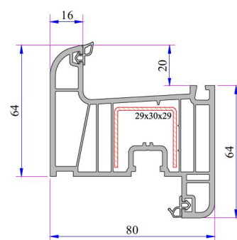
Sash Profile
