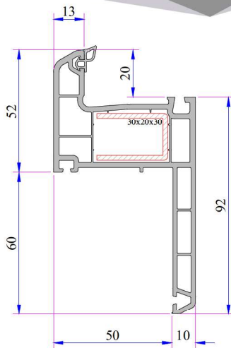
Frame Profile With Sill 60mm
