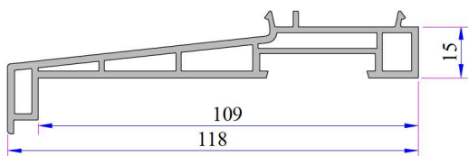
Sill Profile
