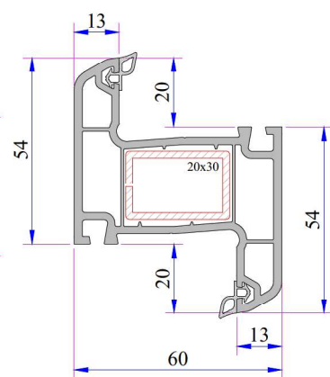
Outward Opening Mullion Profile Code: P.A.632.3005.600.0.BC.03
