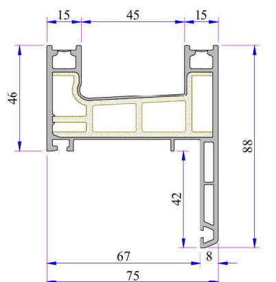
Penwood Frame Profile With Flat Sill Code: ???
