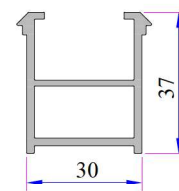
Frame Montage Profile
