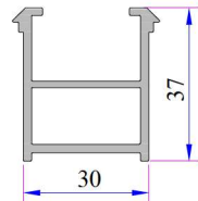
Frame Montage Profile
