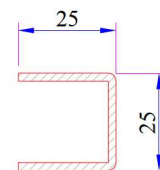
332 Frame- Mullion Profile Reinforcement Code: 34022-12003
