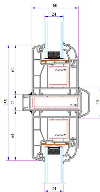
Universal Large Coupling Profile Installation
