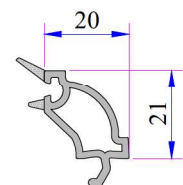
20mm Decorative Glazing Bead Code: P.A.101.4102.600.0.HC
