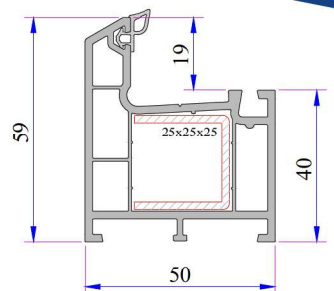
330 Frame Profile
