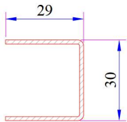
Super Frame - Offset Type Sash Profile Reinforcement
