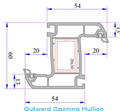
Outward Opening Mullion Profile
