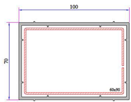
Kutu Profili 70x100mm P.A.070.5202.600.0.00.19
